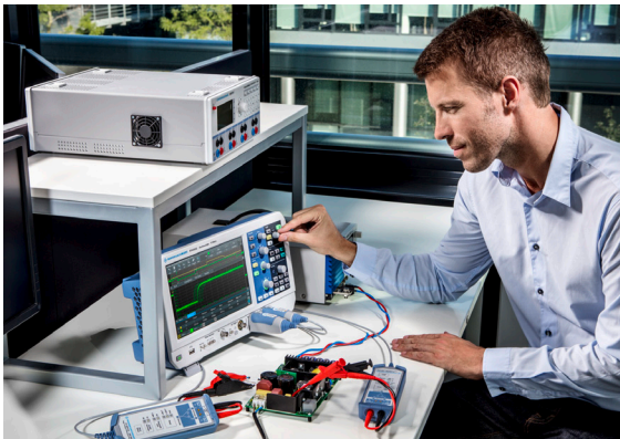
The R&S®RT-ZHD probes safely measure peak voltages up to 6000 V thanks to an industry-leading 2000 V probe offset range and integrated DC voltmeter.
