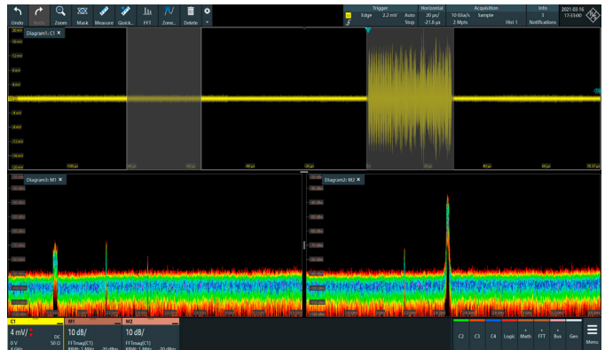
The gated FFT function of the R&S®RTO6 oscilloscope applies FFT analysis only to user-defined regions of the acquired time domain signal.
