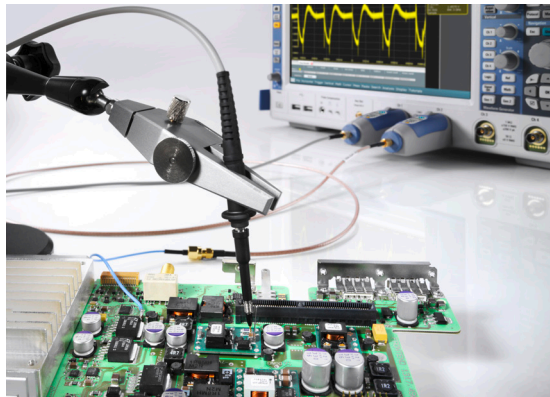
With a bandwidth up to 4.0 GHz, excellent sensitivity thanks to the 1:1 attenuation ratio and low noise, R&S®RT-ZPR probes excel at precise ripple measurements.
